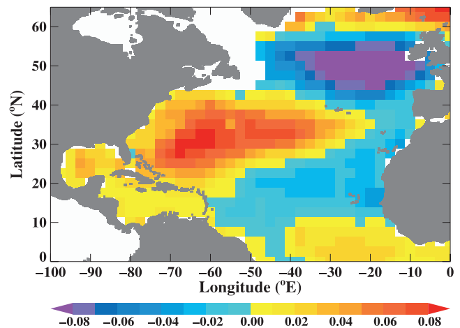
Figure 1. The two orthogonal spatial modes, (a) EOF2 and (b) EOF5, of north Atlantic standardized JJASO mean SST anomalies whose time series are linked significantly and quasi-stably to upcoming NAO DJF indices. The modes are shown for the period 1950–2000. The colour bar shows the sign and normalised strength of the spatial pattern.
